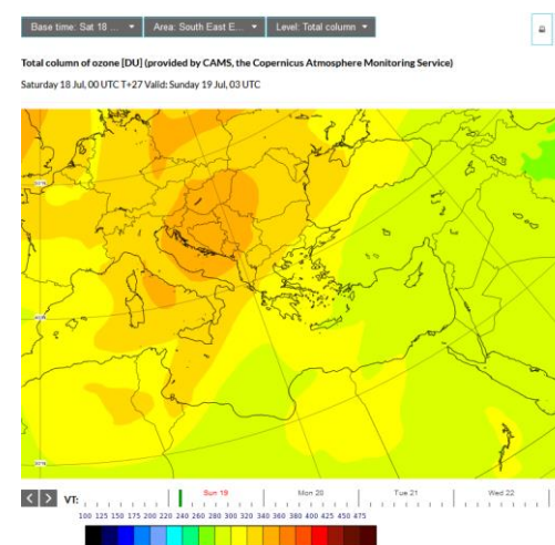
O 3 total column
