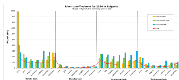
Figure 3. River runoff volume of the low streamflow period in 2024 as compared with a dry, a normal and a wet years chosen
