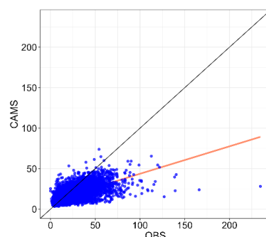
Figure 2. Scatter plot of PM 10 concentrations
