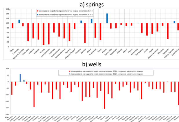
Figure 3. Change in water levels and discharge – October 2024
