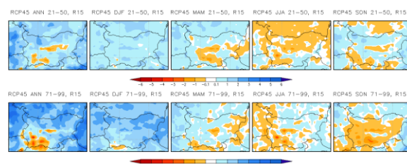
Figure 4. As in Figure 1, but for RCP4.5
