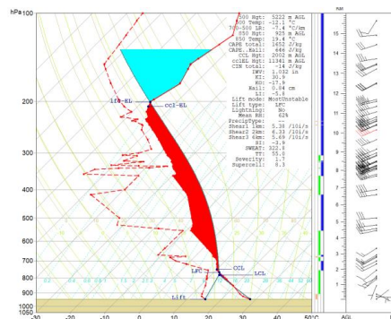
Figure 2. Aerological diagram from June 13, 2024, at 15:00 LT
