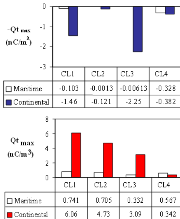
Figure 1. Maximum density of Q_{t\max} ( \text{nC/m}^3 ) of the negative charge (upper panel) and positive charge (lower panel) for the four clouds (CL1, CL2, CL3, and CL4), with different CCN typical for maritime air mass (white columns) and continental air mass (coloured columns)
