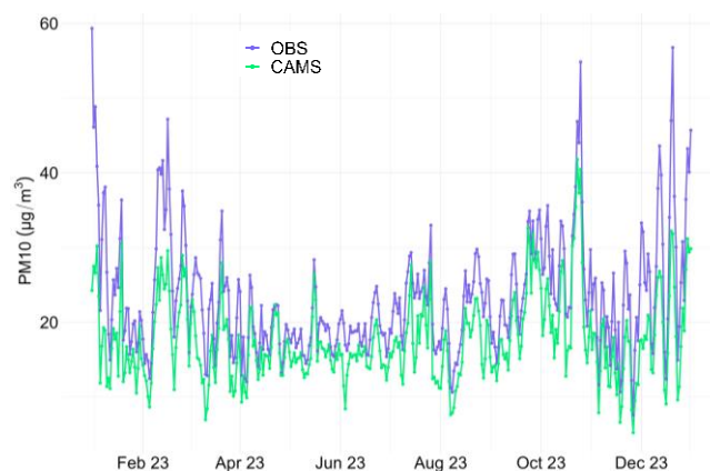
Figure 1. Time series plot of observed and modelled PM 10 concentrations, averaged for 34 stations
