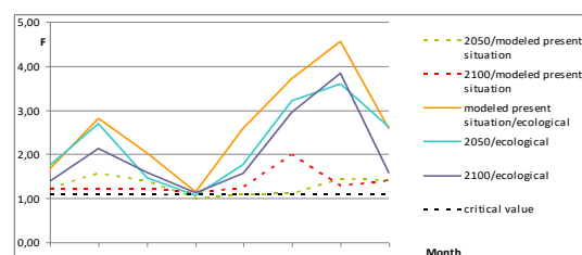
Figure 1. Assessment of the ecological runoff for climate scenarios (Zaharieva, 2020)
