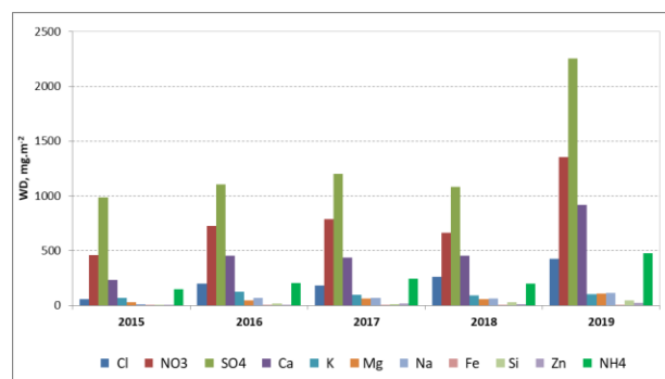
Figure 2. Deposition (WD) of the studied elements for the period 2015–2019
