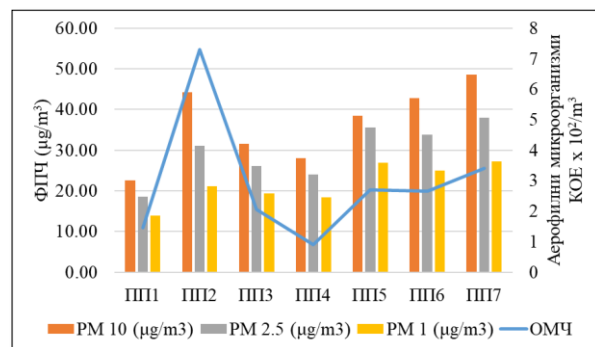
Figure 1. Concentration of PM and TMN
