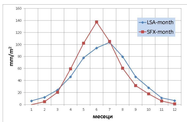
Figure 1. Comparison of average monthly evaporation for Bulgaria from SURFEX and LSA-SAF product
