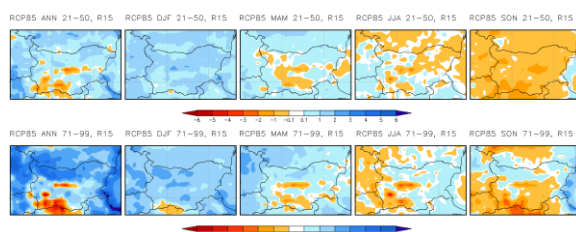
Figure 3. Annual (first column) and seasonal (from the second to the fifth column) change in the number of days/year with precipitation exceeding 15 mm/24 h according to the RCP8.5 scenario for the periods 2021–2050 (first row) and 2071–2099 (second row)
