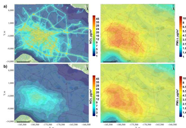
Figure 1. Annual mean concentration for the main transport-related pollutants – NO 2 and PM 2.5 , obtained by using models (a) MAQS with a resolution of 100 m and (b) CMAQ with a resolution of 1 km
