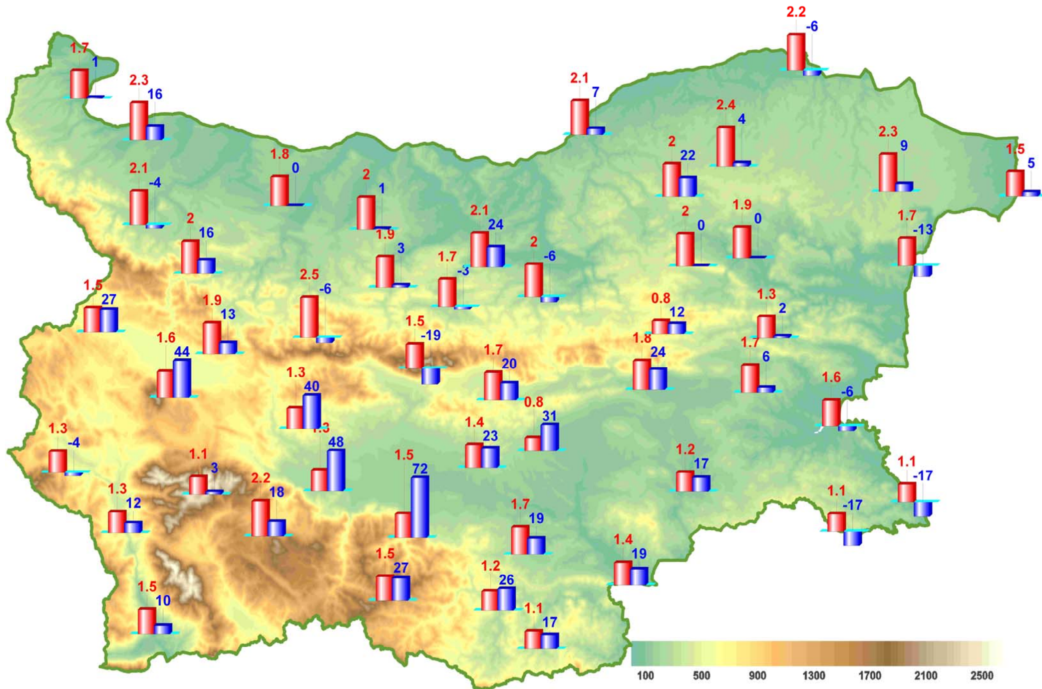
Deviations of annual average air temperature (in °C) and annual precipitation (in %) in 2007, relative to the climate normals for the period 1961-1990
